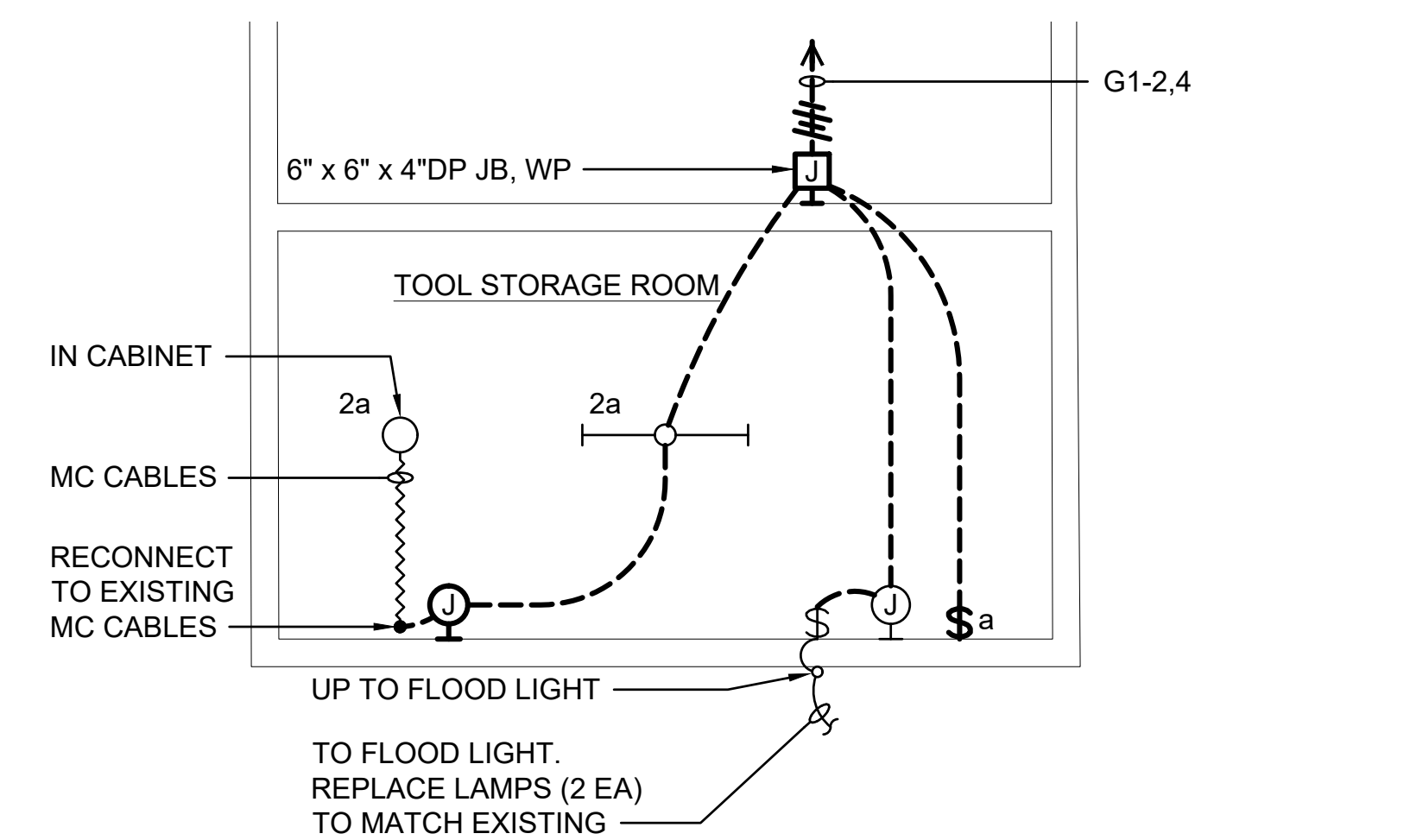
2 TOOL STORAGE ROOM ENLARGED PLAN SCALE: 1/4" = 1'-0" NOTES: 1. LIGHT LINES DENOTE EXISTING CONDITION BOLD LINES DENOTE NEW WORK
