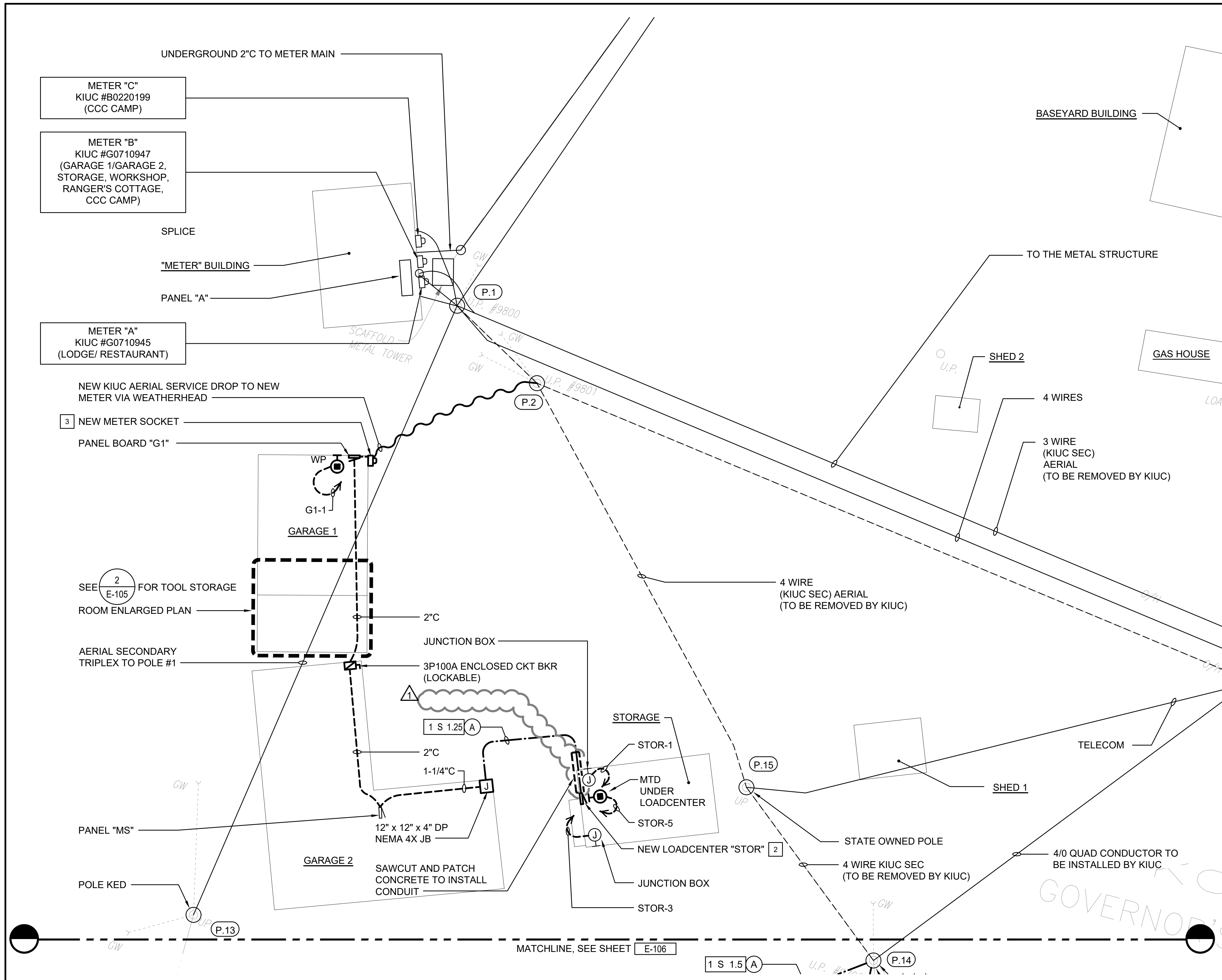
1 ELECTRICAL PLAN A (GARAGES AND STORAGE) SCALE: 1" = 10'-0"
