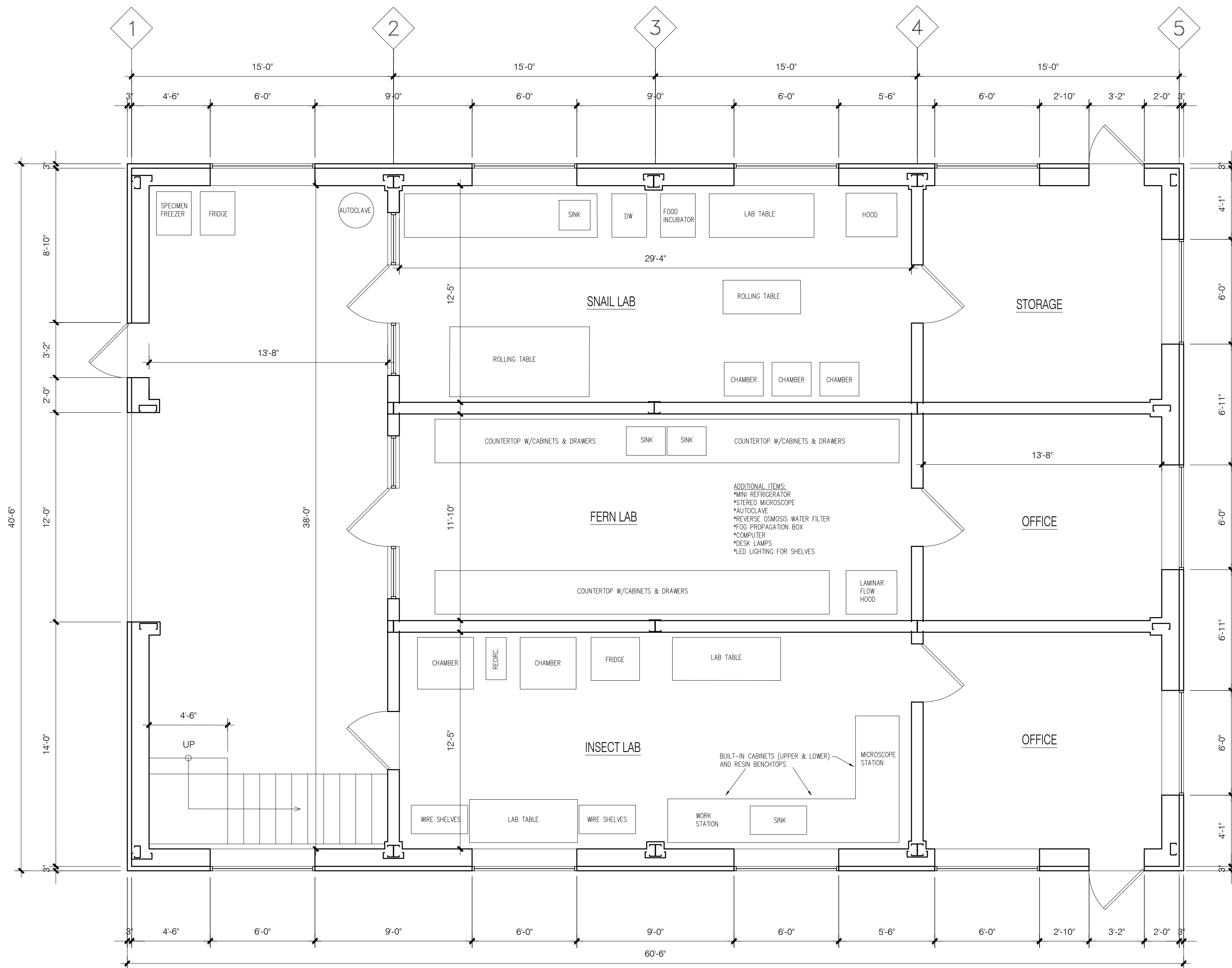
1 A1 OLINDA LABORATORY - MAIN FLOOR PLAN SCALE: 1/4" = 1'-0"
